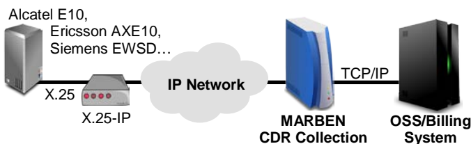
1) CDR collection on IP Backbone
