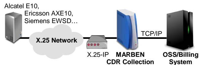
2) CDR Collection on X.25 Backbone
